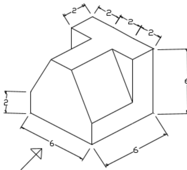
ISOMETRIC PROJECTION
