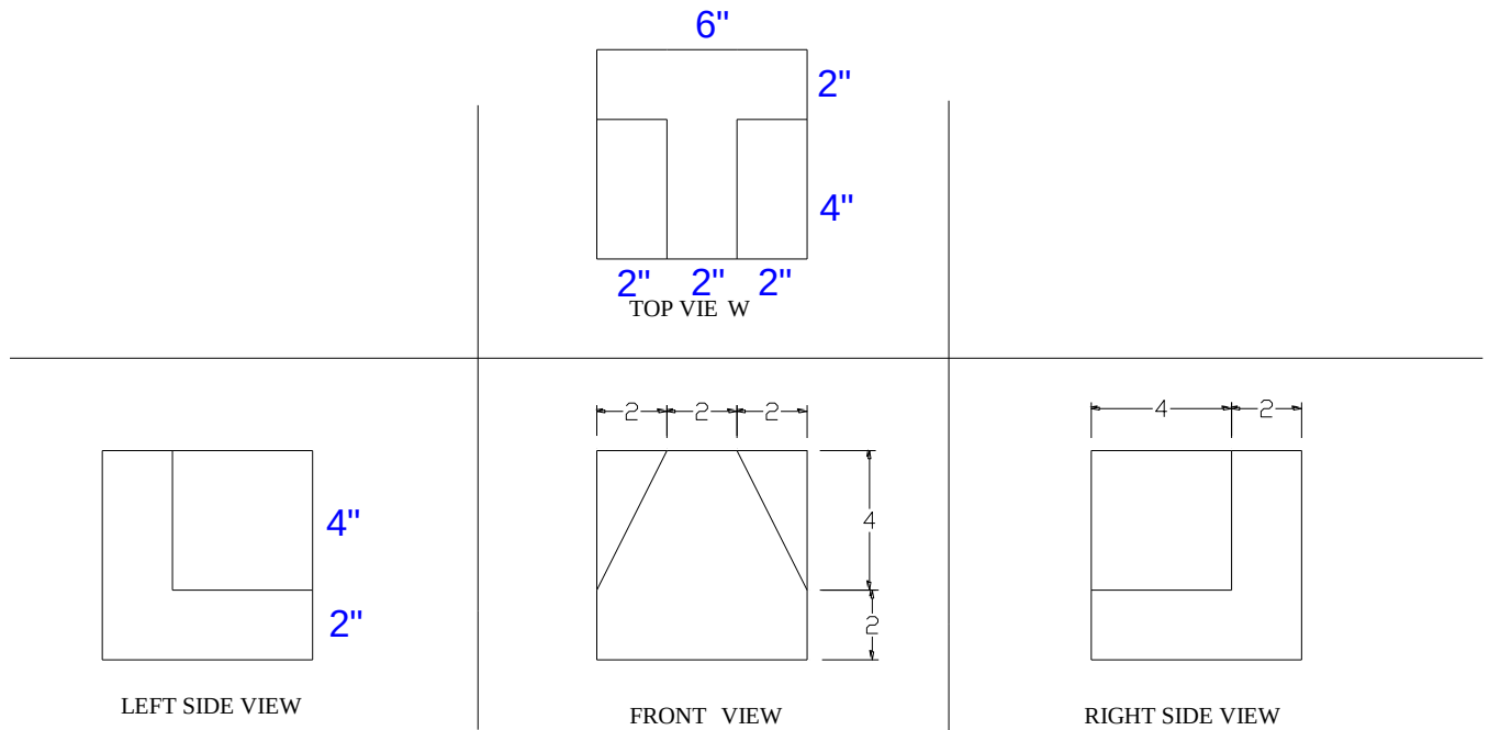
ORTHOGRAPHIC PROJECTION
